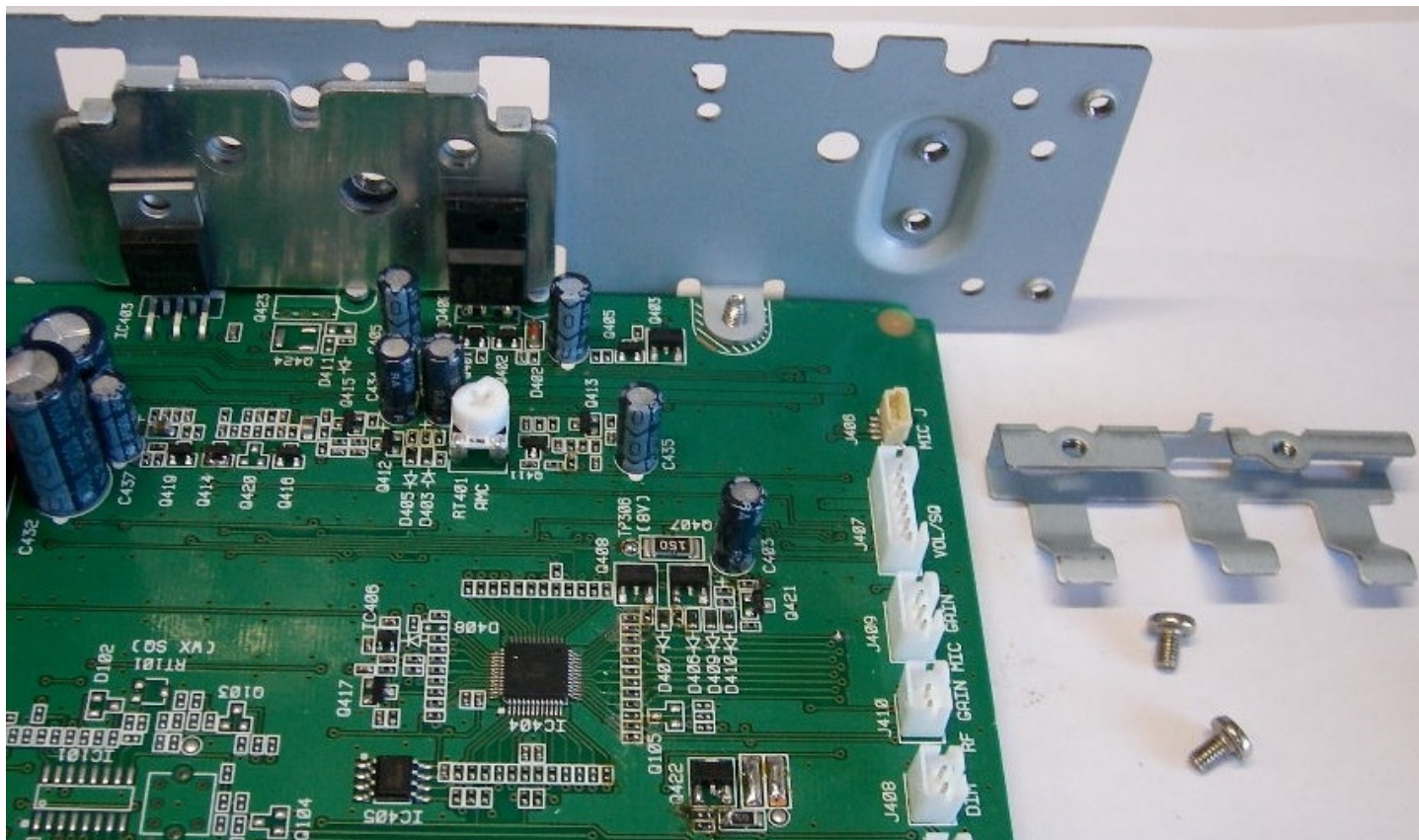
Figure E13.9 – Internal Photo – PCB – Audio Amplifier Section – Heat Sink Removed
