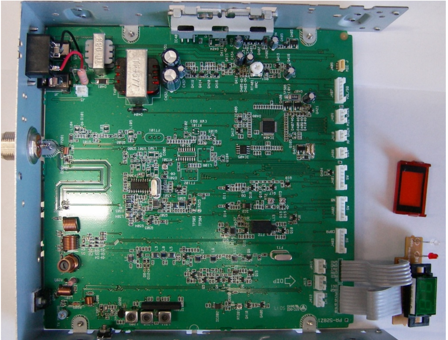
Figure E13.6 – Internal Photo – PCB – Top View
