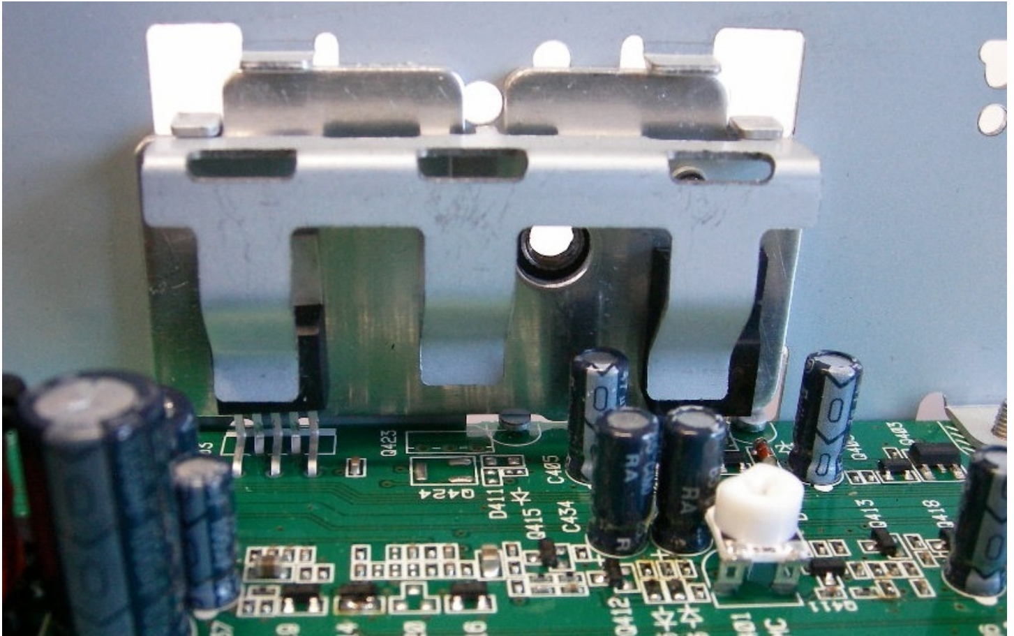
Figure E13.8 – Internal Photo – PCB – Audio Amplifier Section
