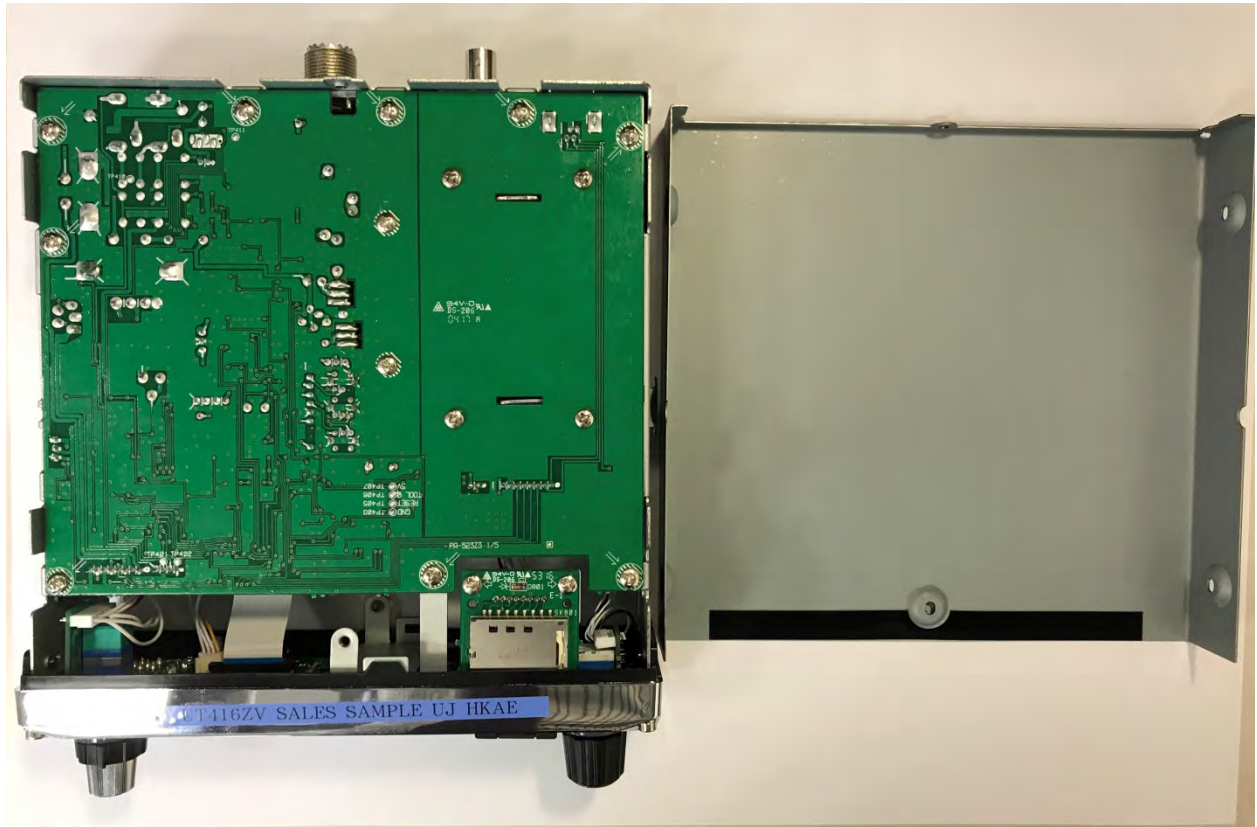
MAIN BOTTOM VIEW WITH COVER
