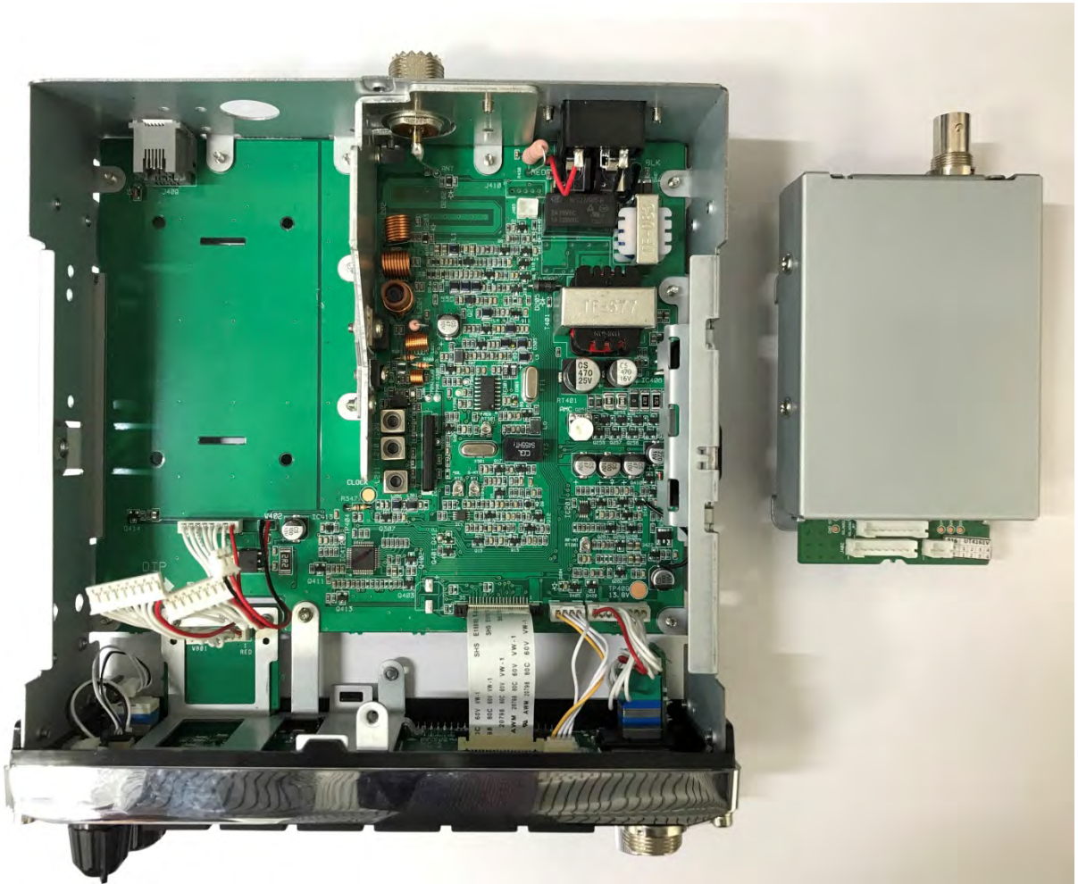
MAIN SCAN TOP VIEW
