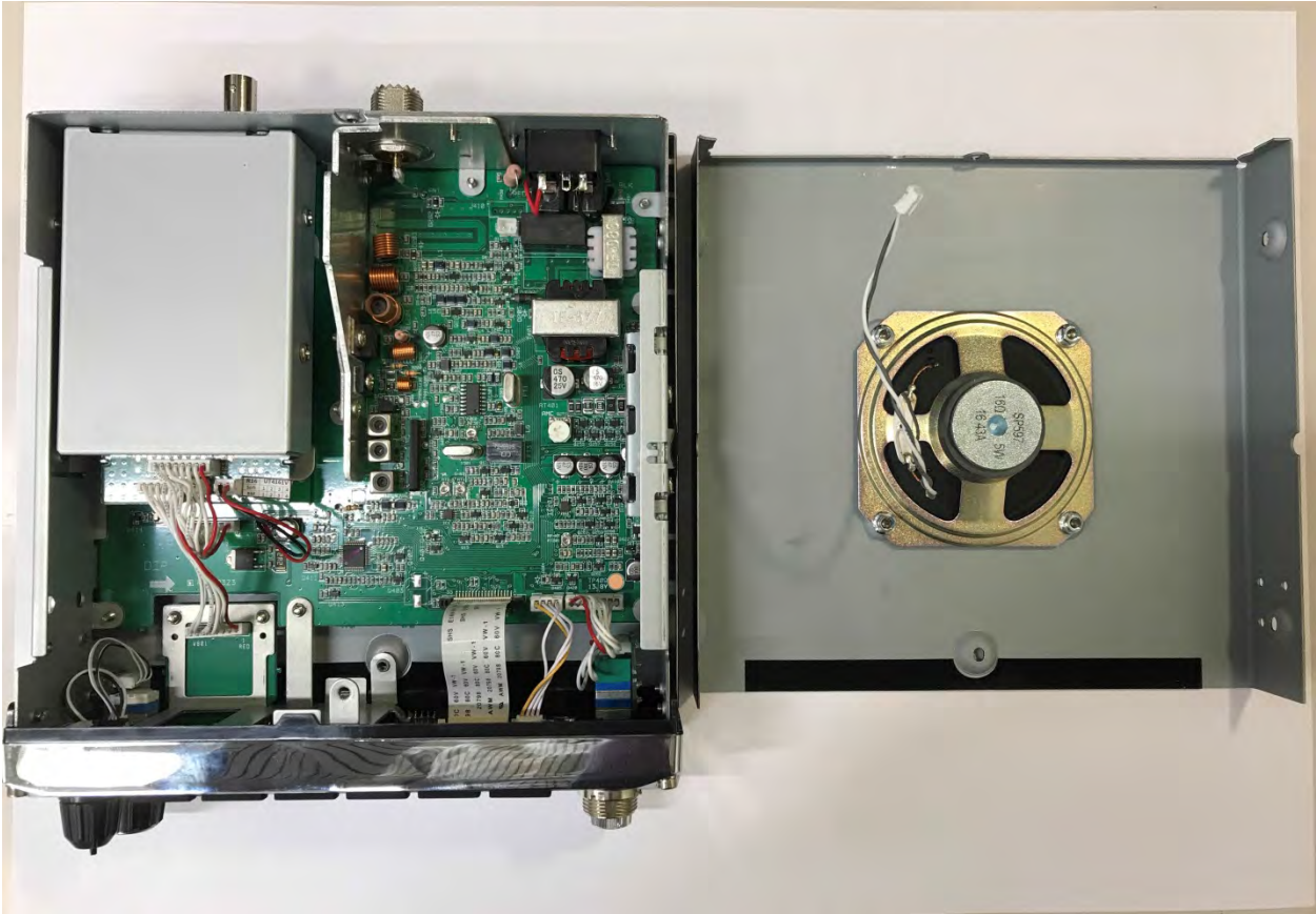
MAIN TOP VIEW – WITH COVER
