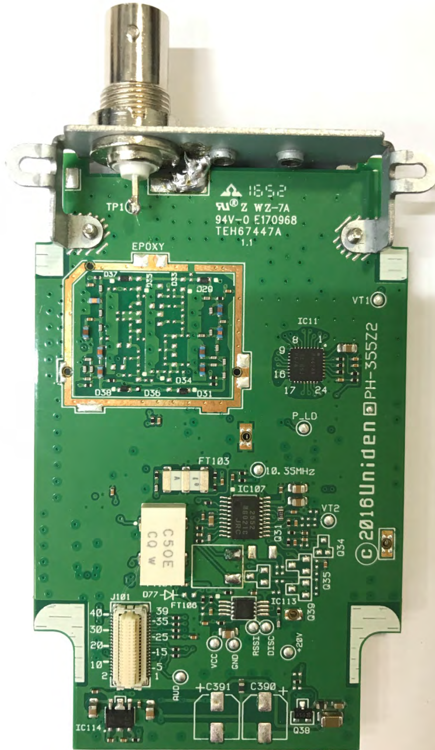
RF BOTTOM VIEW 2
