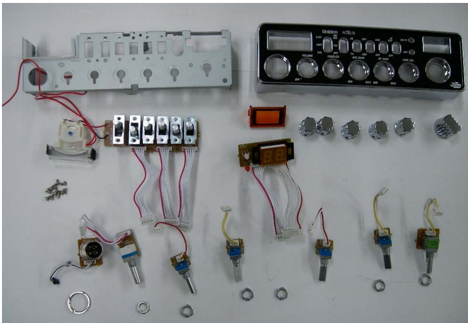
PC78LTD – Front Control Panel Exploded View
