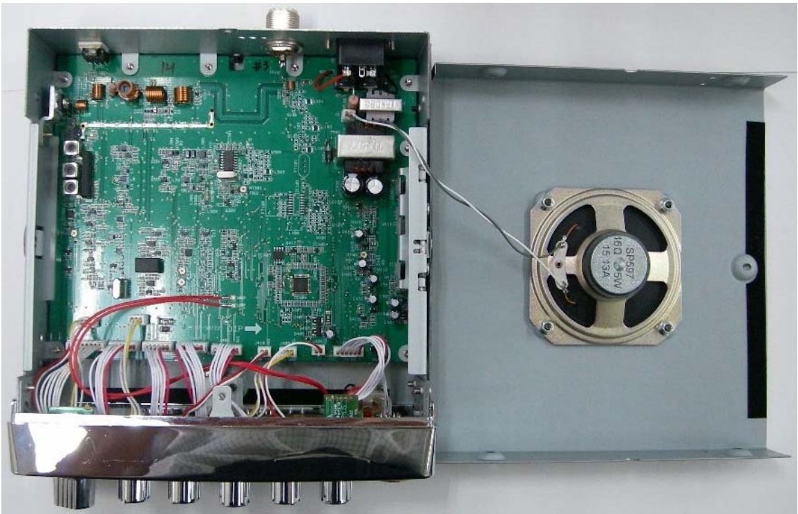
PC78LTD – Main Top View w/ Speaker Wiring
