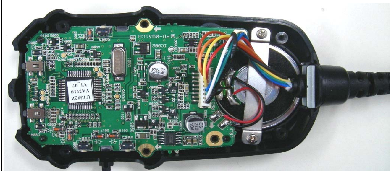
Remote MIC PCB Top View
