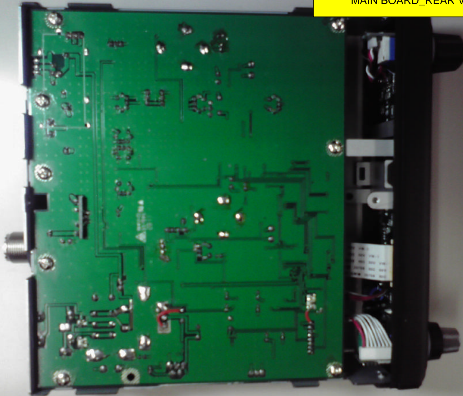
MAIN BOARD_REAR VIEW
