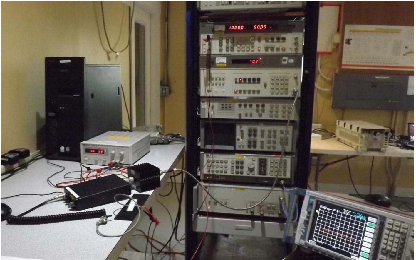
Figure E23.2 – Setup, Audio Response
