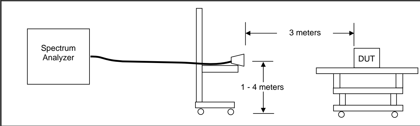
Figure F.6-1 - Setup Drawing – Radiated TX Spurious Emissions
