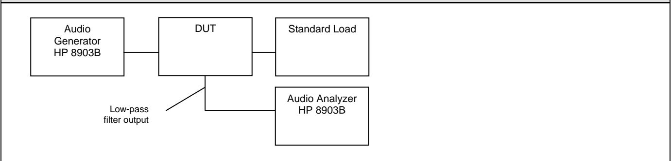
Figure D.5-1 - Setup Drawing – Low-pass Filter Response
