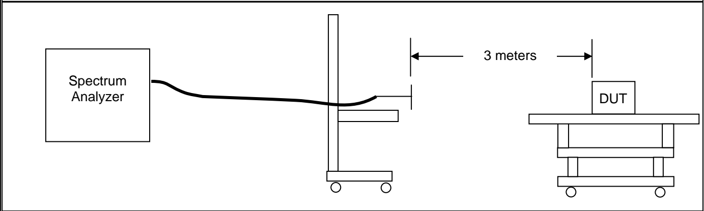
Figure A.5-1 - Setup Drawing – RF Output Power
