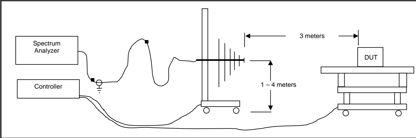
Figure G.6-1 - Setup Drawing – Radiated RX Spurious Emissions
