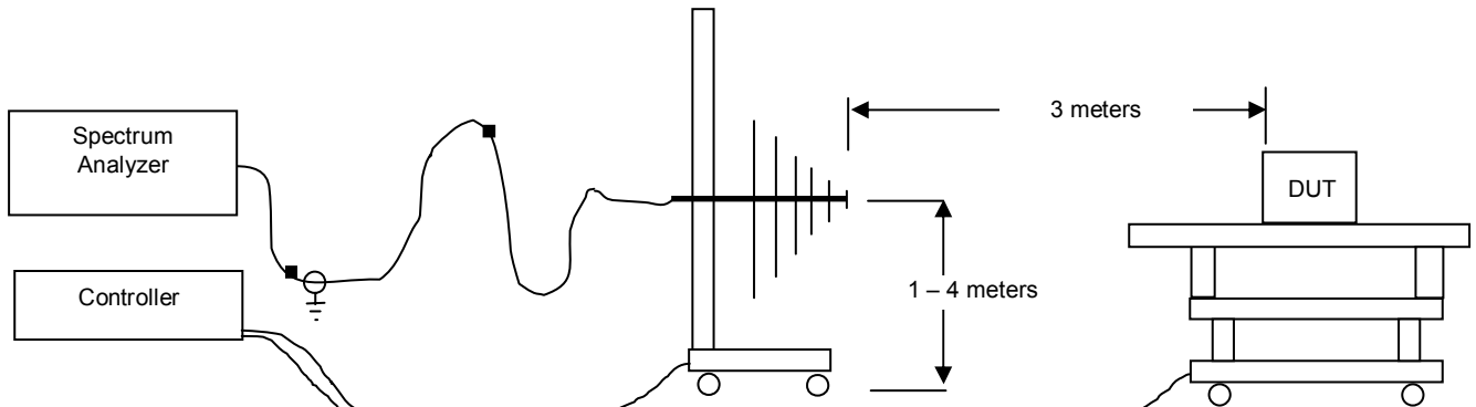
Figure G.6-1 - Setup Drawing – Radiated RX Spurious Emissions
