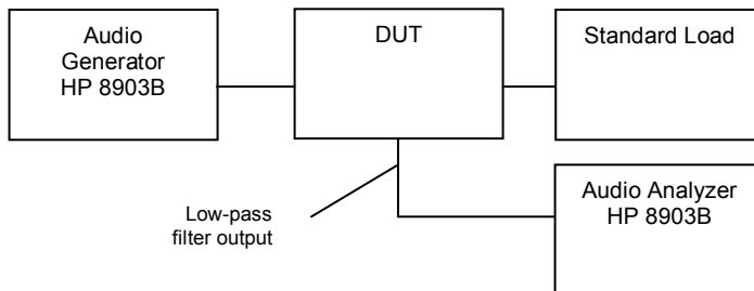
Figure D.5-1 - Setup Drawing – Low-pass Filter Response
