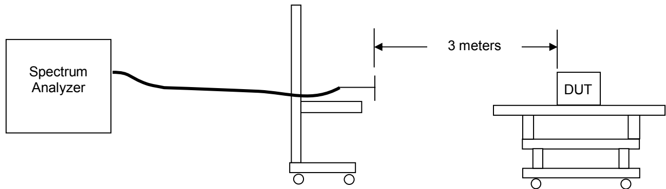
Figure A.5-1 - Setup Drawing – RF Output Power
