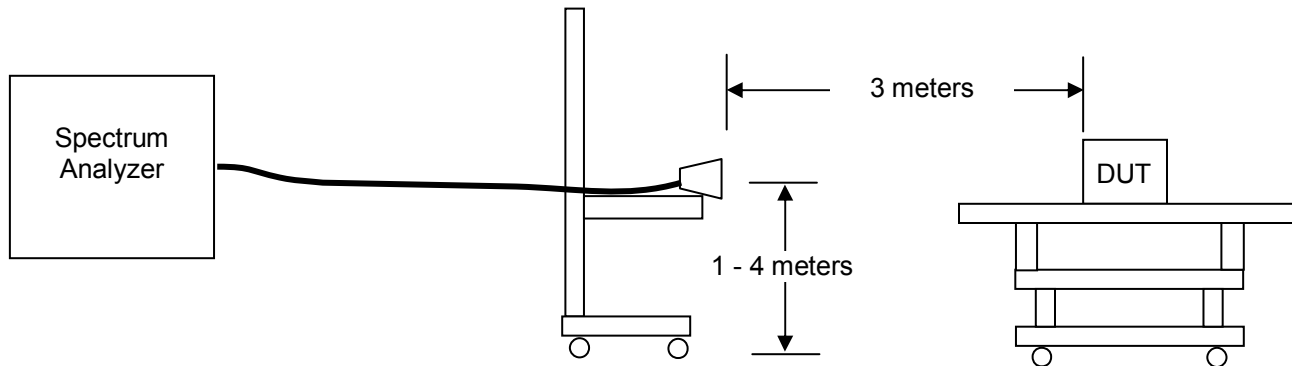
Figure F.6-1 - Setup Drawing – Radiated TX Spurious Emissions
