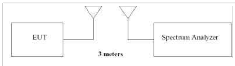
Figure A-3. Test Instrument & Measurement Setup
