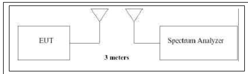
Figure A-2 Test Instrument & Measurement Setup
