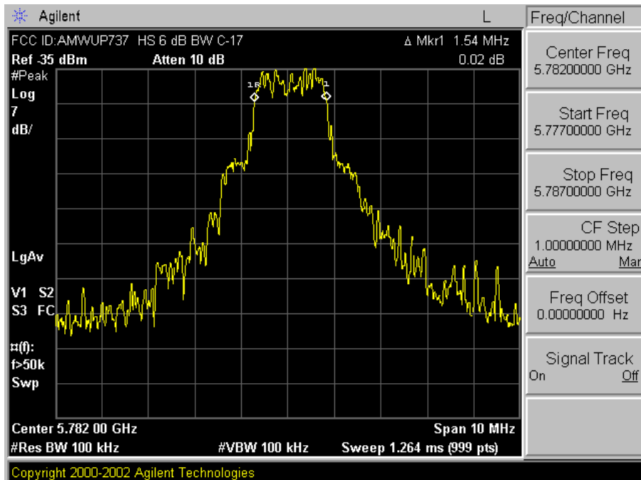
Plot A-2. 6dB Bandwidth Plot – Ch. 17 (HS)
