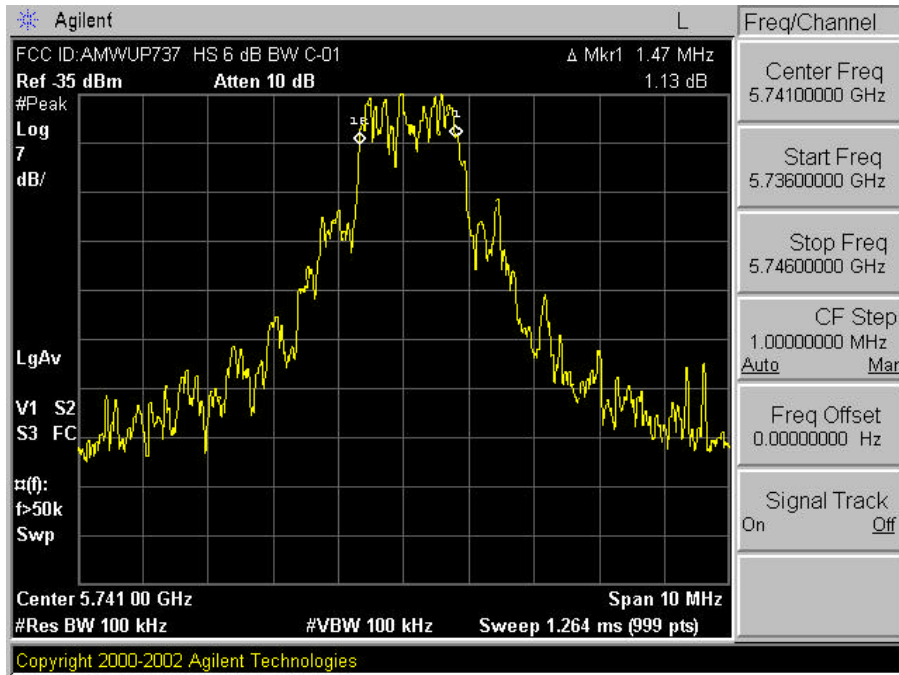
Plot A-1. 6dB Bandwidth Plot – Ch. 01 (HS)
