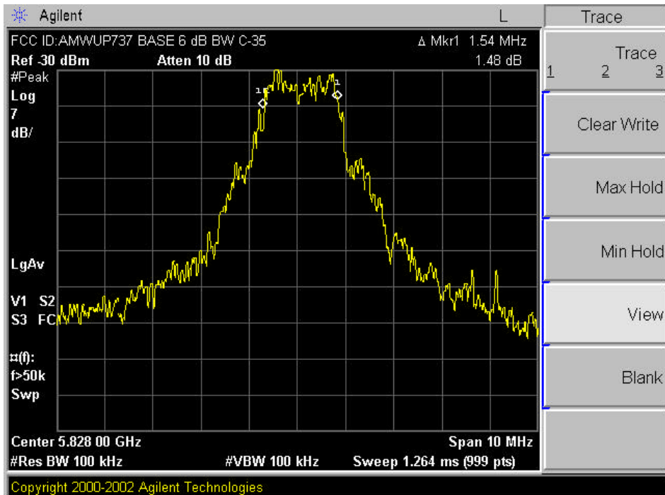
Plot A-2. 6dB Bandwidth Plot – Ch. 17 (BASE)
