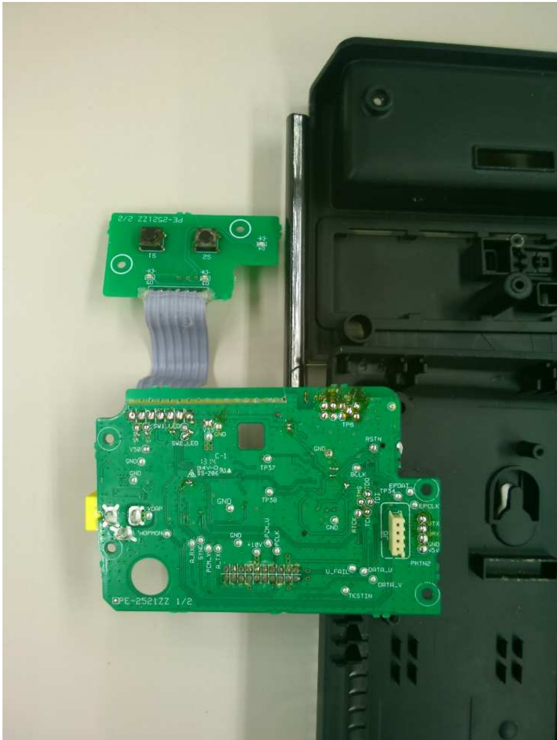
Main PCB Bottom View & Key PCB Top View [ “EXP11000” Base]
