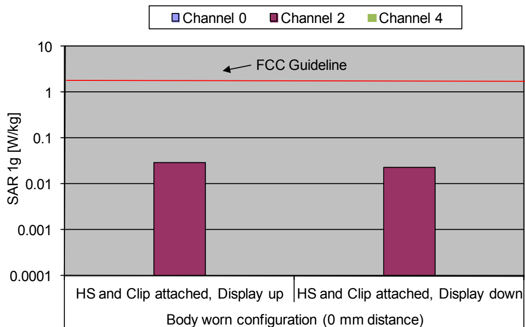
Fig. 9: The measured SAR values in body worn configuration for the Avaya D160 for the US DECT standard in comparison to the FCC exposure limit.
