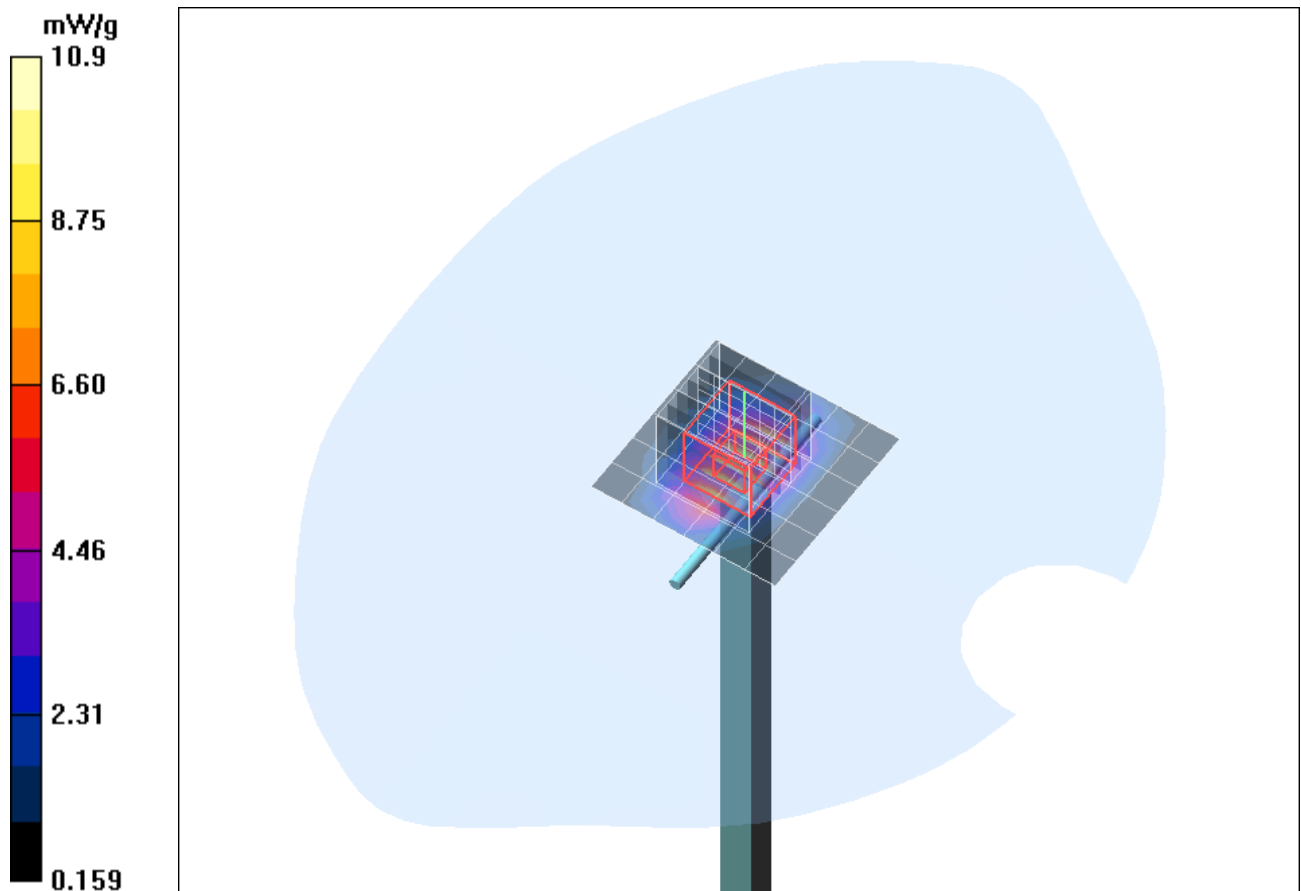
Fig. 11: Validation measurement 1900 MHz body (June 11, 2012), coarse grid. Ambient Temperature: 21.5° C, Liquid Temperature: 21.3° C.
