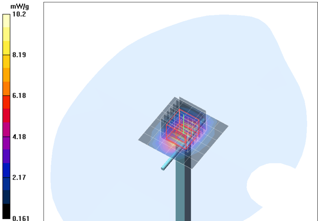
Fig. 10: Validation measurement 1900 MHz Head (May 29, 2012), coarse grid. Ambient Temperature: 22.0° C, Liquid Temperature: 21.8° C.
