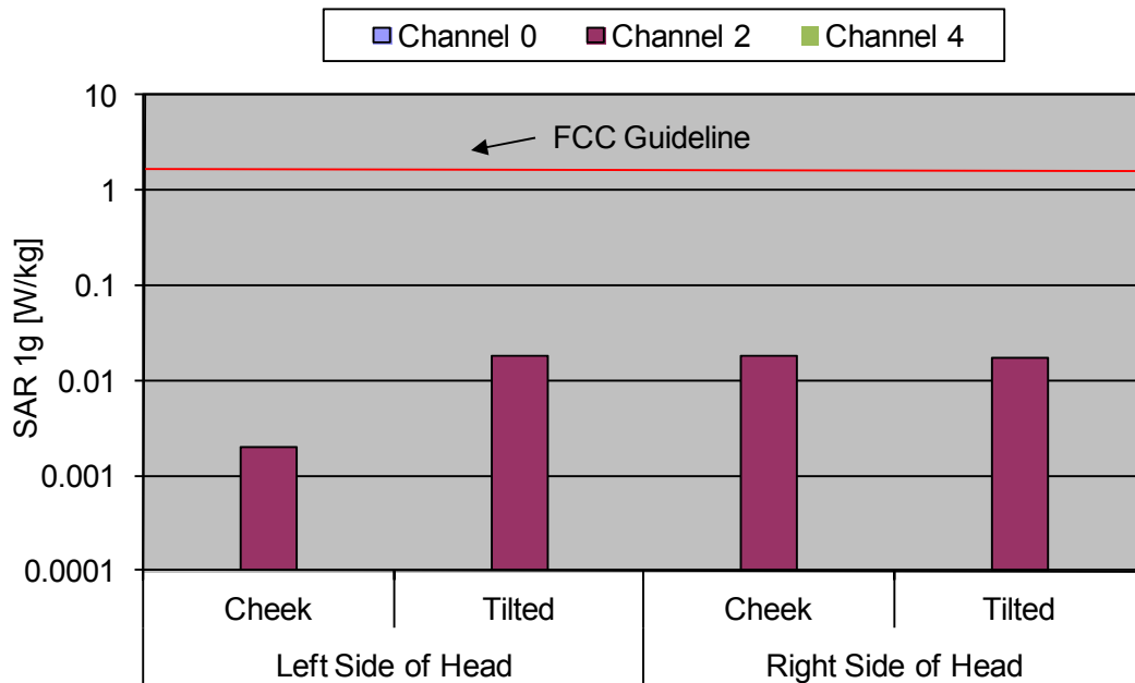
Fig. 8: The measured head phantom SAR values for the Avaya D160 for the US DECT standard in comparison to the FCC exposure limit.
