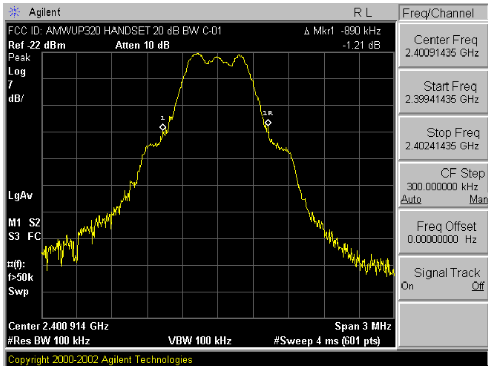
Plot A-1. 20dB Bandwidth Plot – Ch. 01 (Handset)
