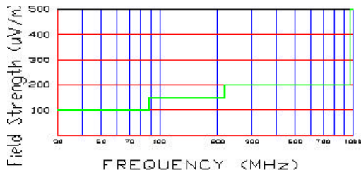
Figure A-9. Radiated limits at 3 meters.
