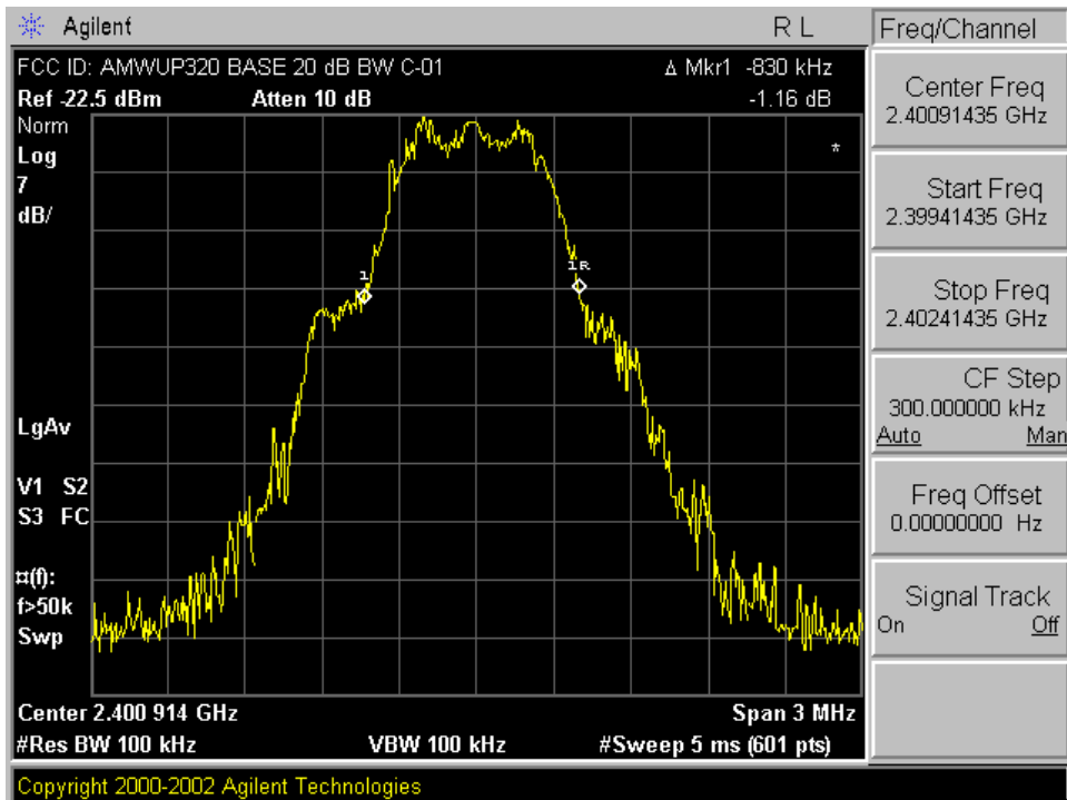
Plot A-4. 20dB Bandwidth Plot – Ch. 01 (Base)
