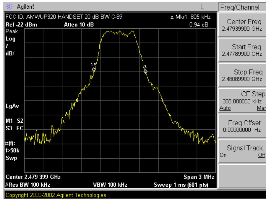
Plot A-3. 20dB Bandwidth Plot – Ch. 89
