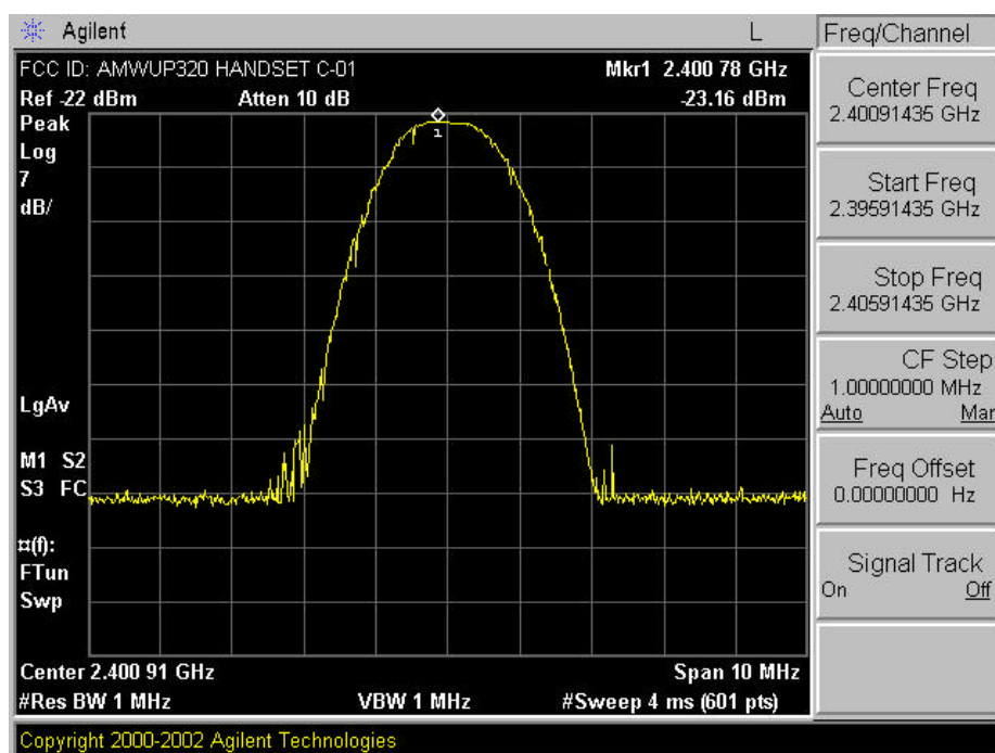
Plot A-4. Max. Peak Output Power Plot – Ch. 01 (Handset)
