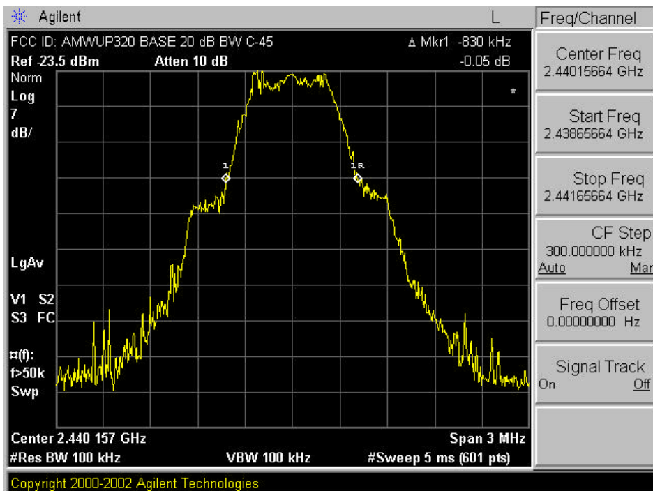
Plot A-5. 20dB Bandwidth Plot – Ch. 45 (Base)
