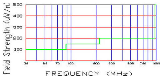
Figure A-17. Radiated limits at 3 meters
