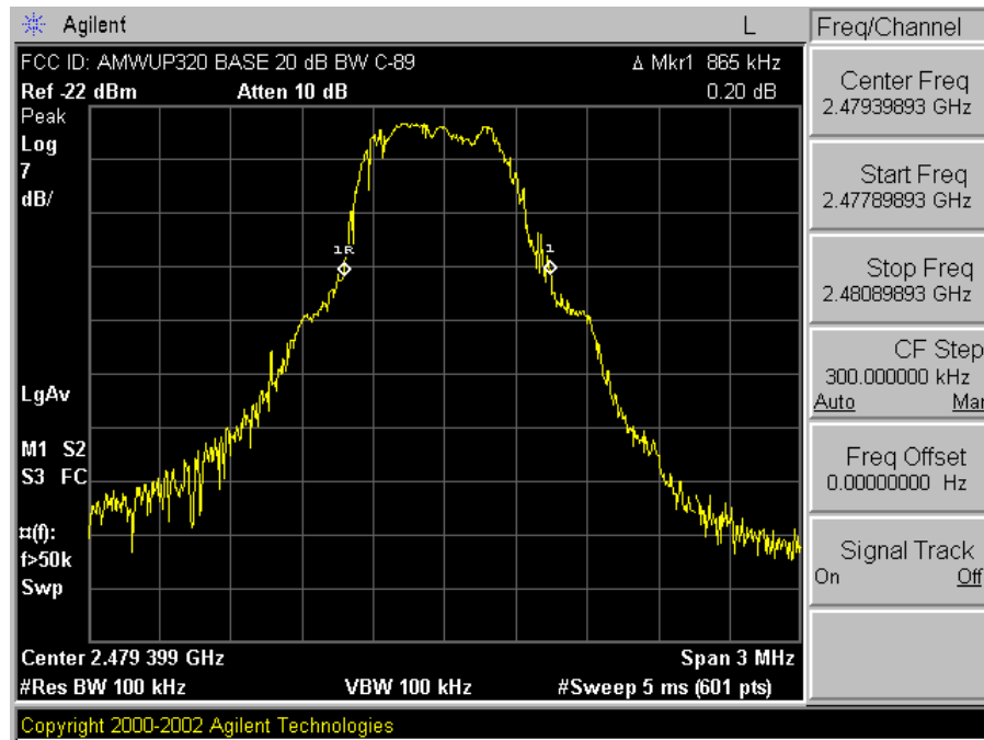
Plot A-6. 20dB Bandwidth Plot – Ch. 89 (Base)
