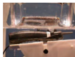
Figure 14.5 Body SAR Test Setup -- w/ Belt-Clip --
