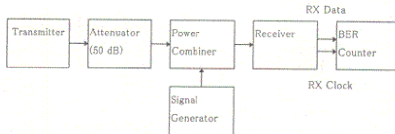
Fig. 5 The test configuration.
