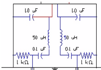
Figure 5. LISN Schematic
