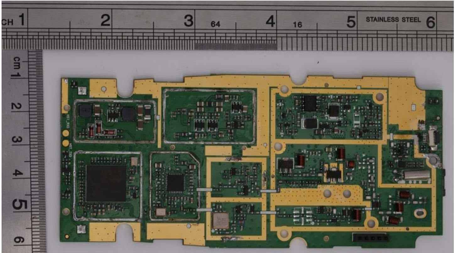
Figure E20.4 – Internal Photo – Heat Sink Removed
