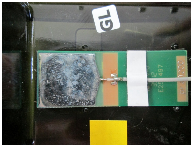
Photograph 7.3.1 Antenna assembly
