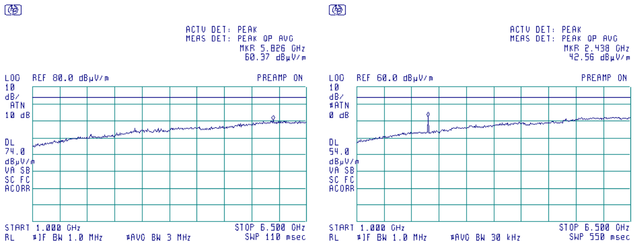
Plot 8.1.4 Radiated emission measurements in 1000 - 6500 MHz range, horizontal antenna polarization
