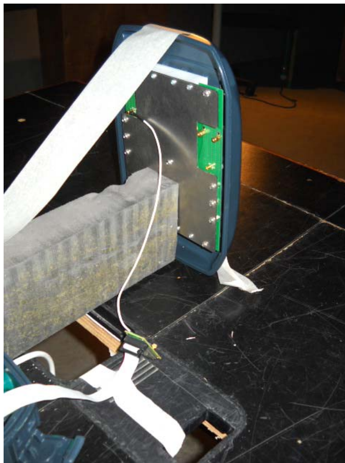
Photograph No.4 Setup for spurious emission field strength measurements in the anechoic chamber, EUT with connected antenna close view
