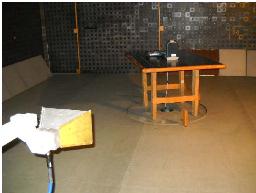
Photograph No.3 Setup for spurious emission field strength and OBW measurements in the anechoic chamber in 1 - 18 GHz range
