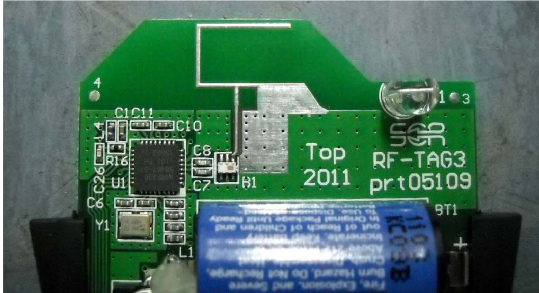
Photograph No.4 H-TAG-LD antenna view
