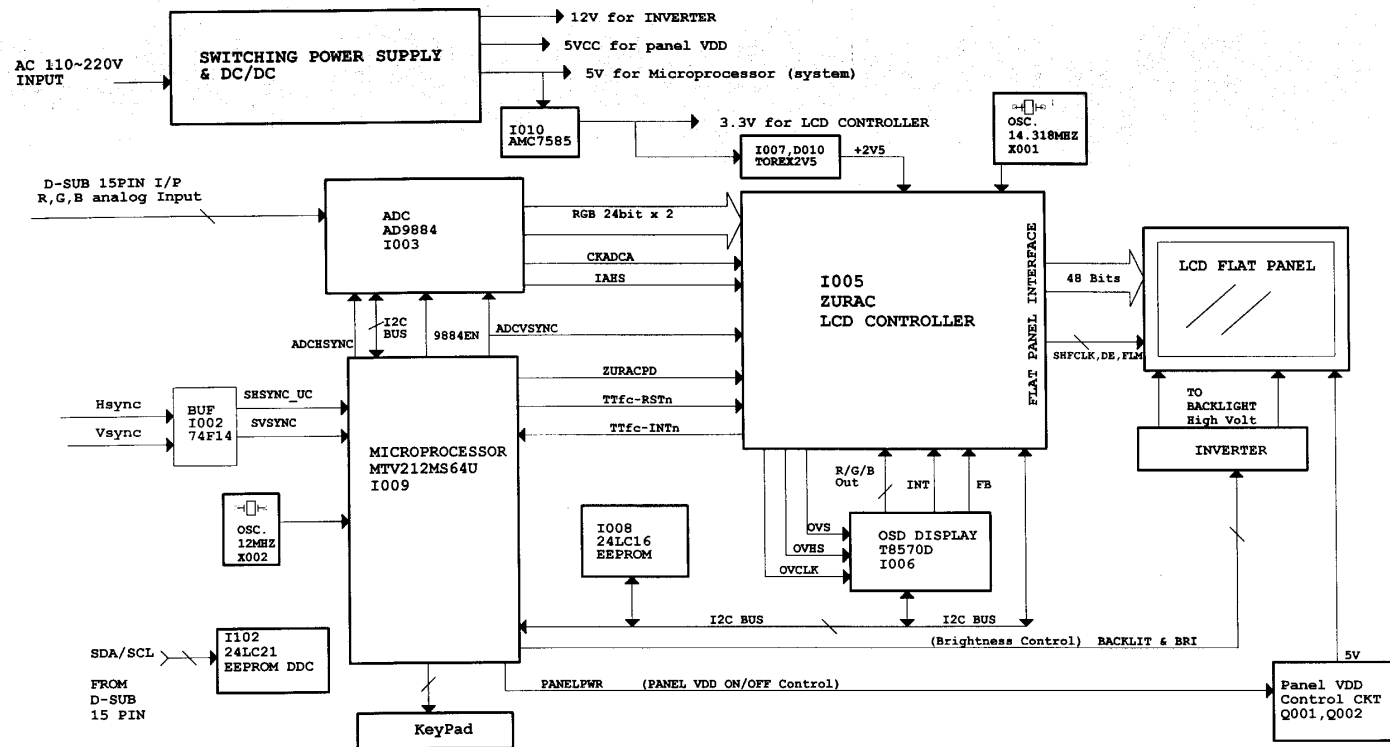
✓ JT186P11 LCD MONITOR FLOW CHAR
