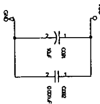
DECOUPLING FOR DIGITAL VCC & VDD OF 8752
