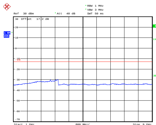
NB-IOT Band 5 CH-Middle 1GHz-9GHz
