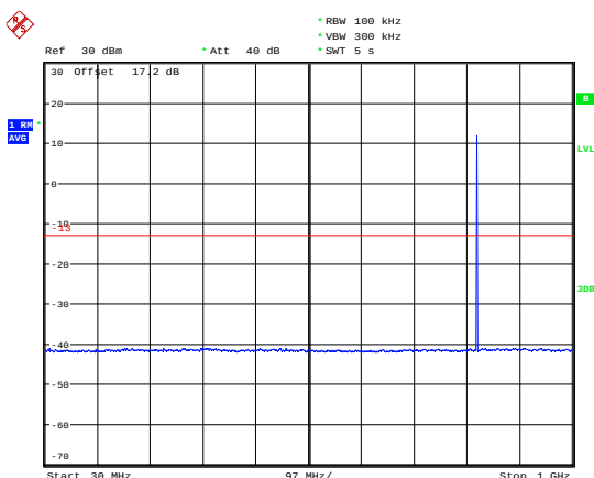
NB-IOT Band 5 CH-Low 30MHz-1GHz
