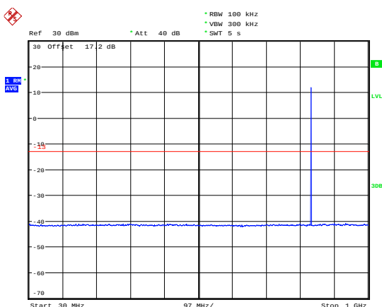
NB-IOT Band 5 CH-Middle 30MHz-1GHz
