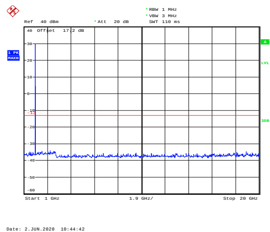
GSM 1900 CH-High 1GHz ~ 20GHz
