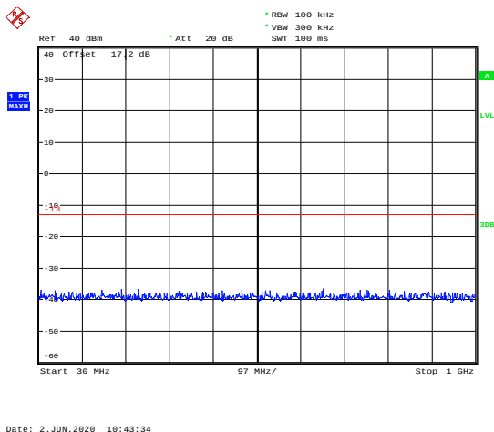
GSM 1900 CH-High 30MHz ~ 1GHz
