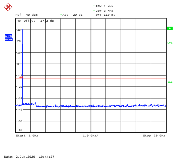
GSM 1900 CH-High 1GHz ~ 20GHz
