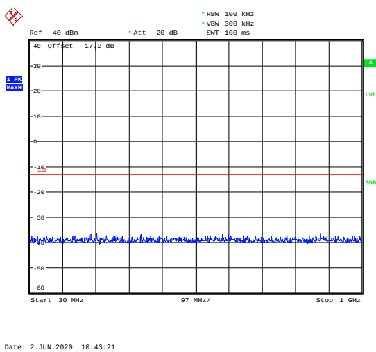
GSM 1900 CH-High 30MHz ~ 1GHz
