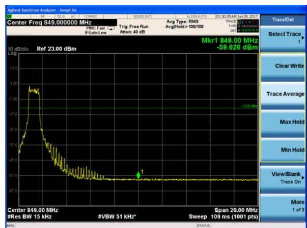
LTE Band 26 16QAM 10MHz CH-High 100%RB
