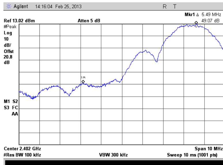
Figure 7.4.1.2-1: Lower Band-edge
