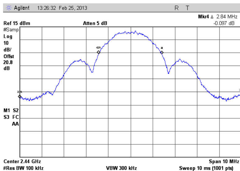
Figure 7.2.2-5: 99% OBW - Middle Channel
