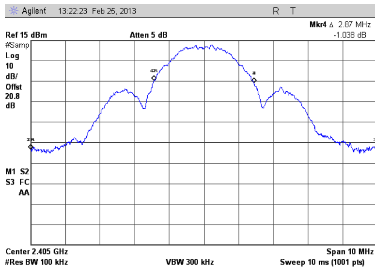
Figure 7.2.2-4: 99% OBW - Low Channel
