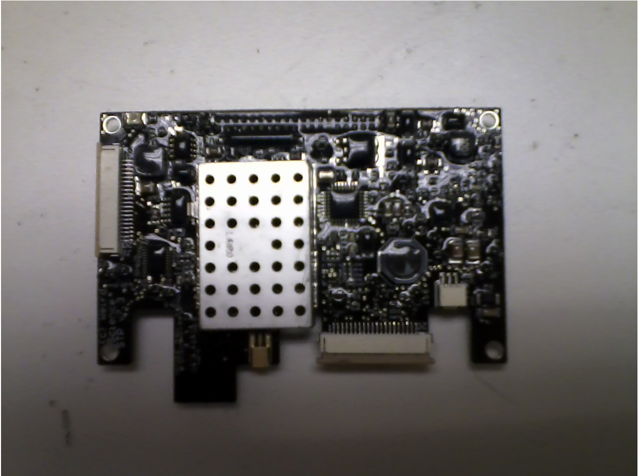
Figure 1: RF Board (Top View with shield)
