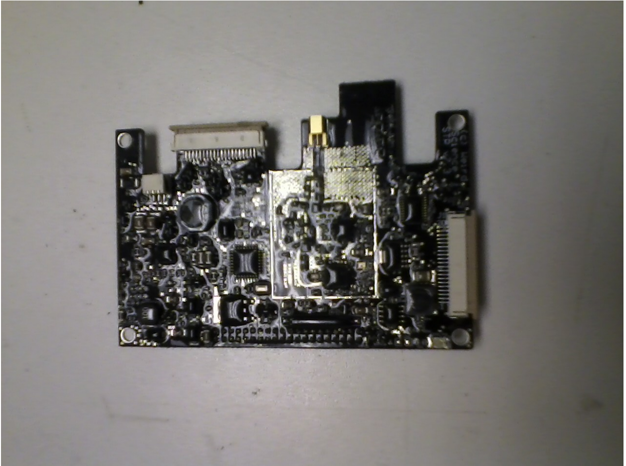
Figure 2: RF Board (Top View without shield)
