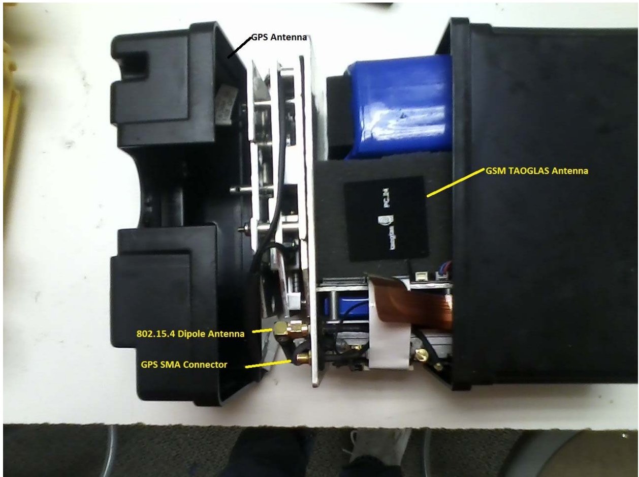
Figure 9: Internal View (Showing GPS, GSM and Zigbee Antennas)
