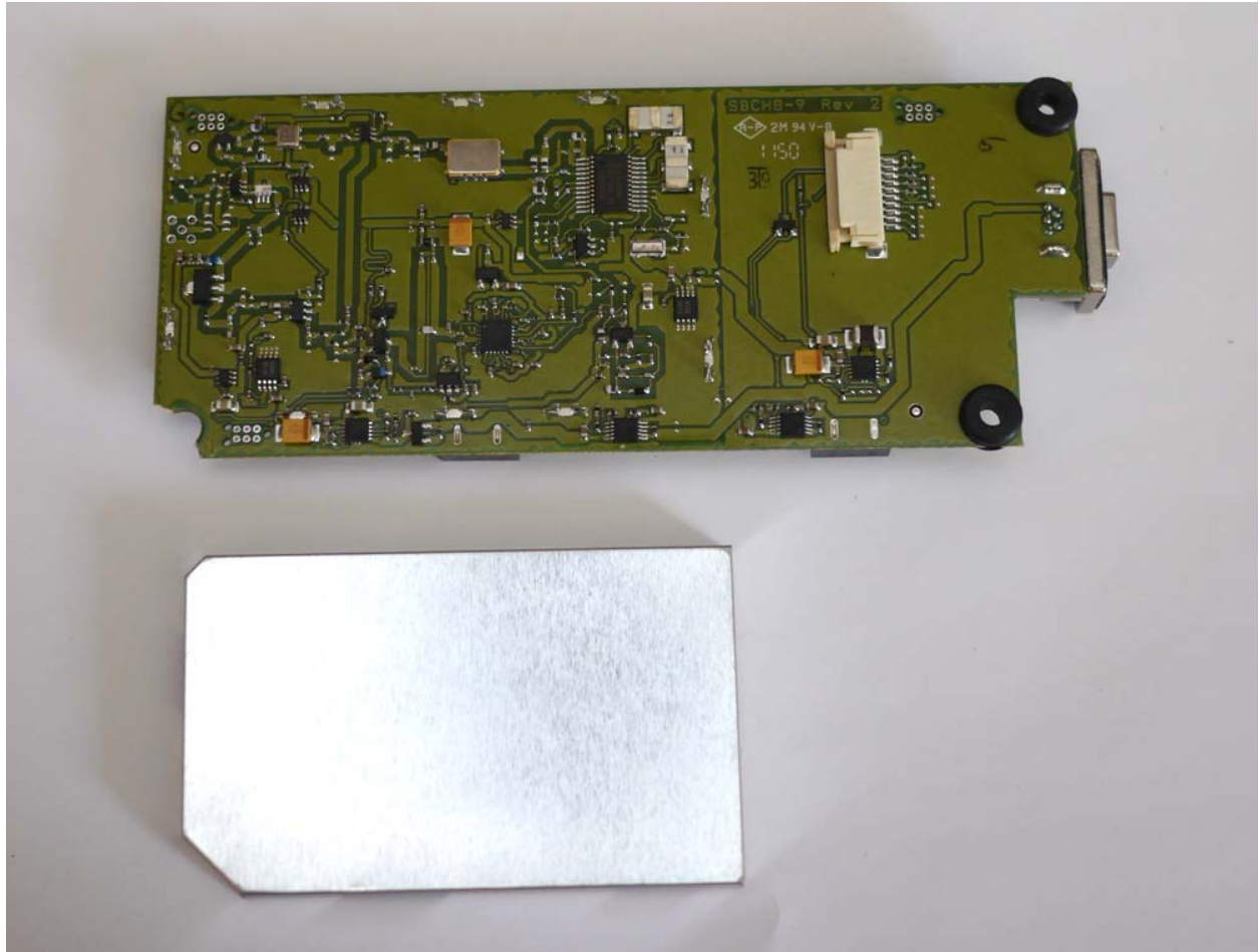
View of the Bottom of the PCB with RF Shield Removed
