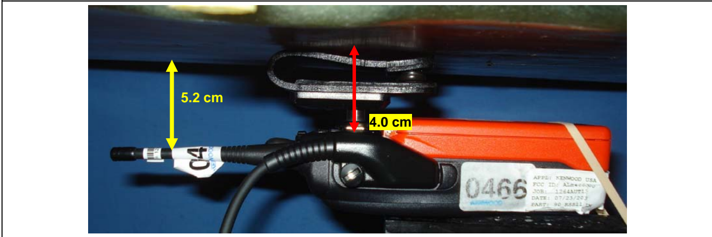
Body-worn SAR Configuration 3 - Antenna 2, Battery e, Audio G1a
