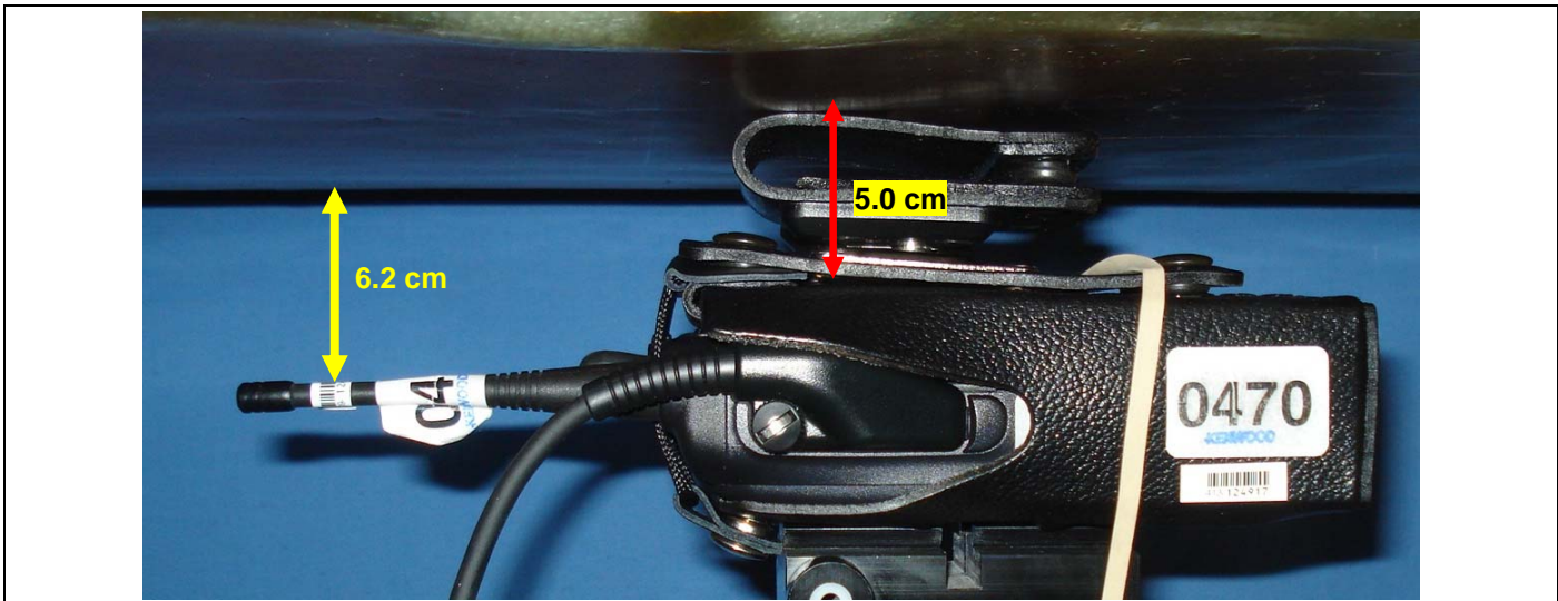
Body-worn SAR Configuration 4 - Antenna 2, Audio G1a
