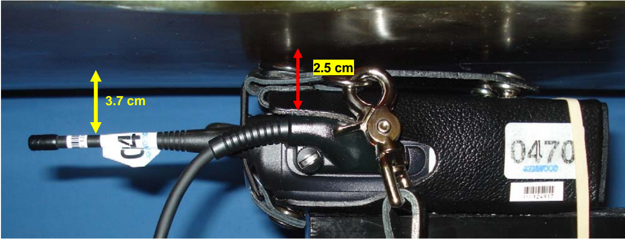
Body-worn SAR Configuration 8 - Antenna 2, Audio G1a
