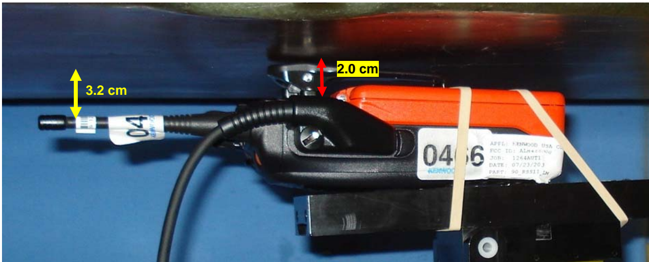
Body-worn SAR Configuration 1 - Antenna 2, Battery e, Audio G1a
