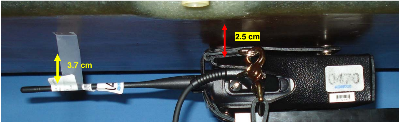
Body-worn SAR Configuration 8 - Antenna 1, Audio G1a
