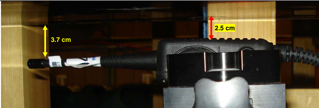
Face-held SAR Configuration - Antenna 1
