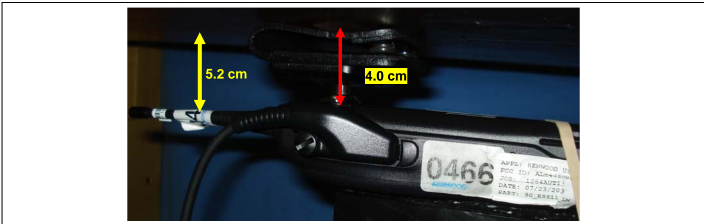
Body-worn SAR Configuration 3 - Antenna 2, Audio G1a
