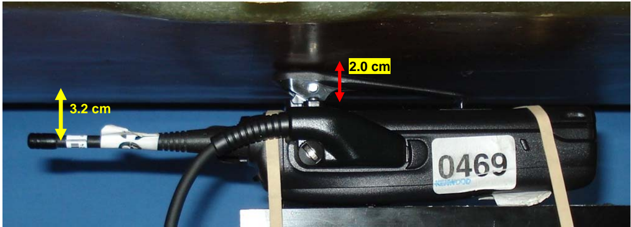
Body-worn SAR Configuration 1 - Antenna 2, Audio G1a
