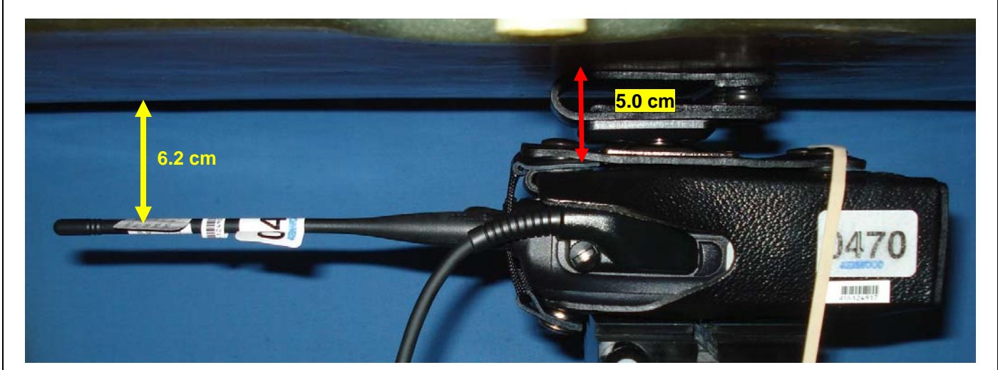
Body-worn SAR Configuration 4 - Antenna 1, Audio G1a
