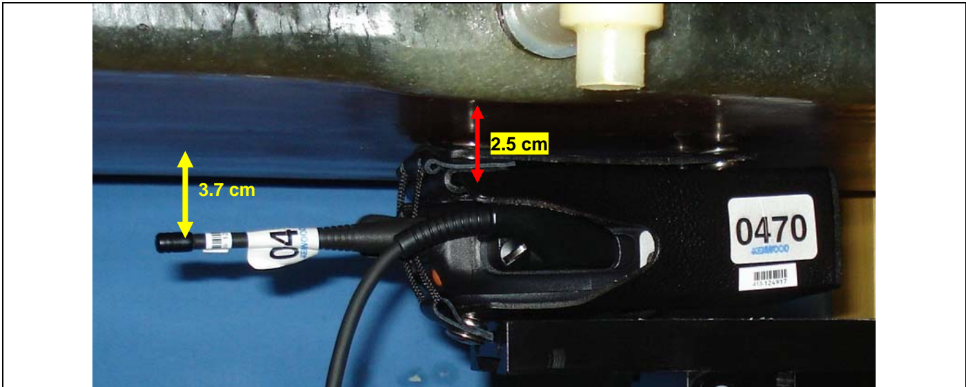
Body-worn SAR Configuration 7 - Antenna 2, Audio G1a
