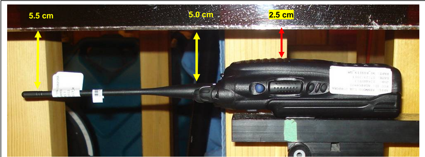
Face-held SAR Configuration - Antenna 1, Battery b
