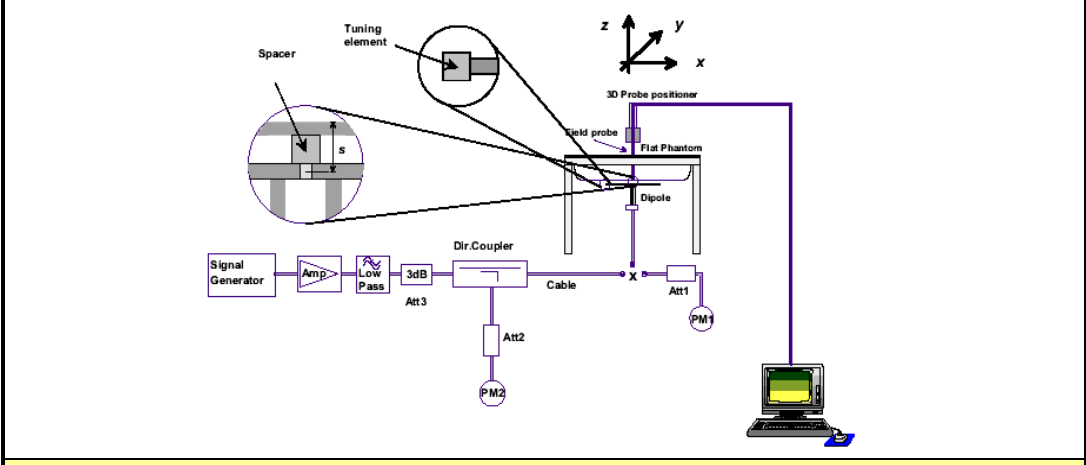
System Performance Check Measurement Setup (IEEE Standard 1528-2003) SPEAG 450 MHz Validation Dipole Setup
