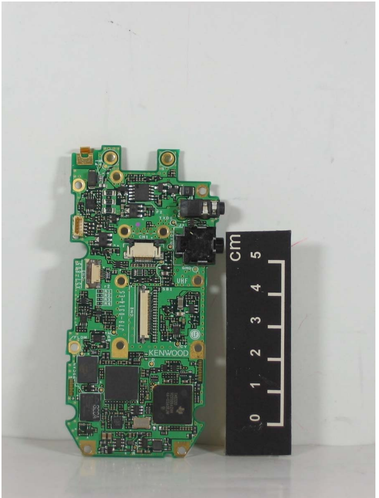
NX-320-K4, NX-320-K5, NX-320-K6 TXRX Unit
