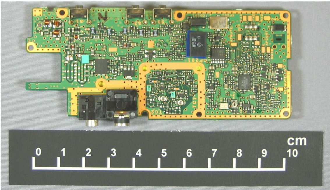
TXRX Component Side View
