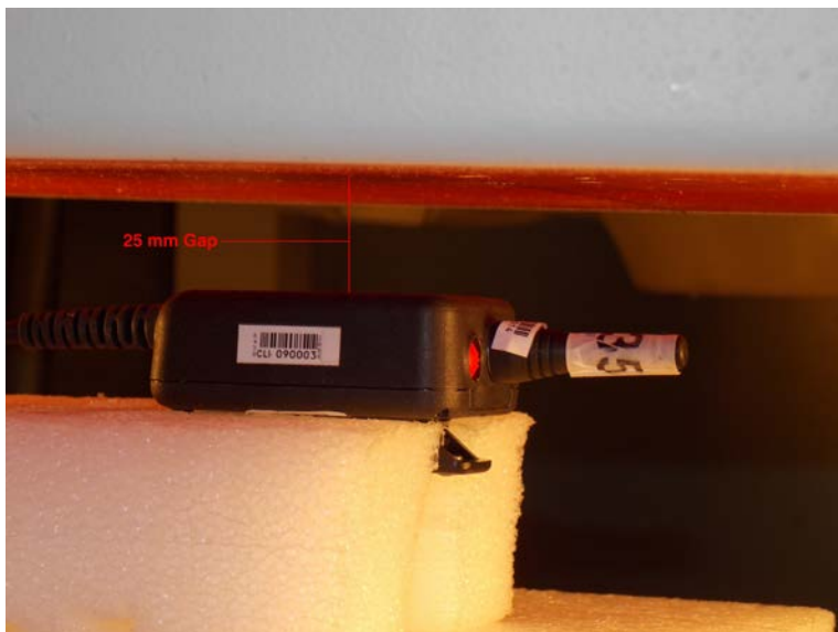
Audio Accessory C with Antenna B Face Configuration
