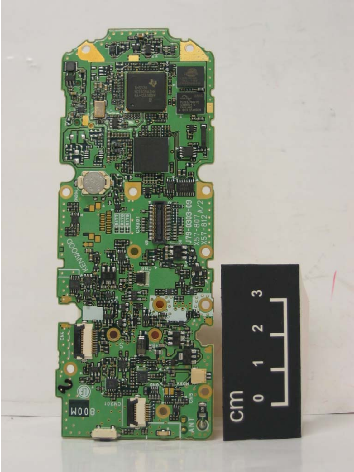
TXRX UNIT
