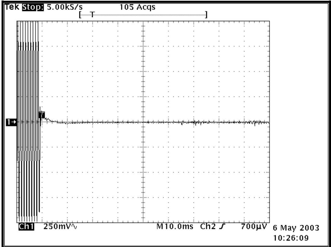
PLOT 13-3: TRANSIENT FREQUENCY BEHAVIOR – 470.15 MHz; HIGH POWER; NARROW BAND; CARRIER ON TIME
