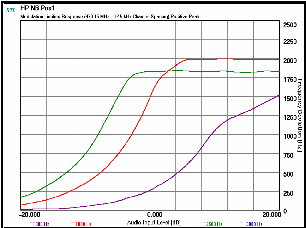
PLOT 12-3: MODULATION CHARACTERISTICS – MODULATION LIMITING: NARROW BAND; POSITIVE PEAK
