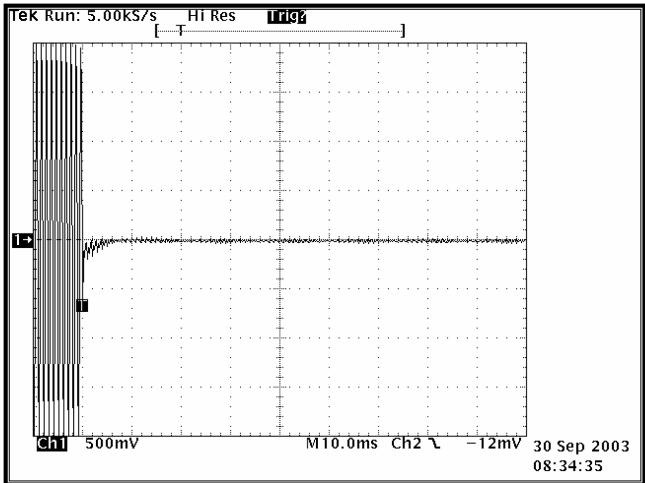
PLOT 13-1: TRANSIENT FREQUENCY BEHAVIOR – 160.15 MHZ; HIGH POWER; WIDE BAND; CARRIER ON TIME
