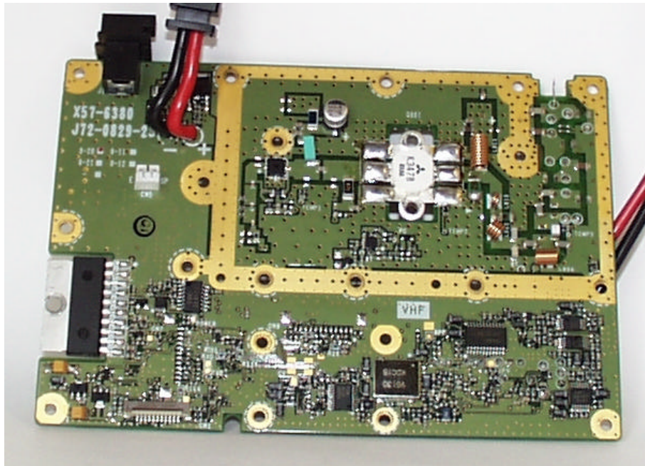
PC Board: Top view
