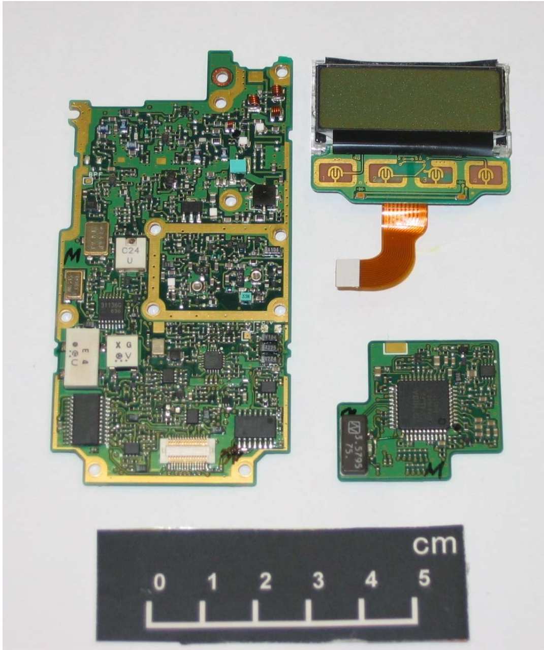
Component Side View
