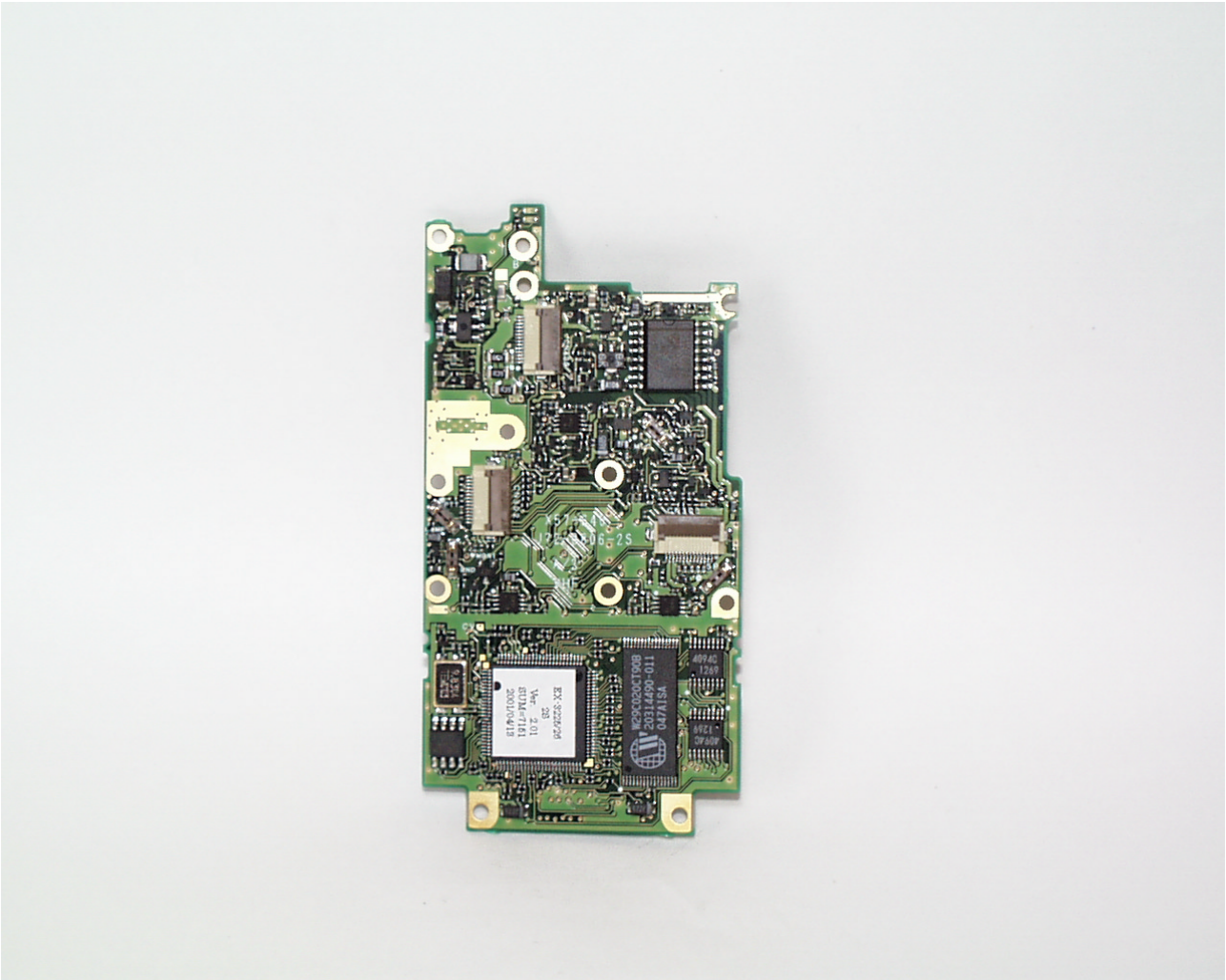
FCC ID: ALH32253110 Model Name: TK-2140K PC Board: Front View
