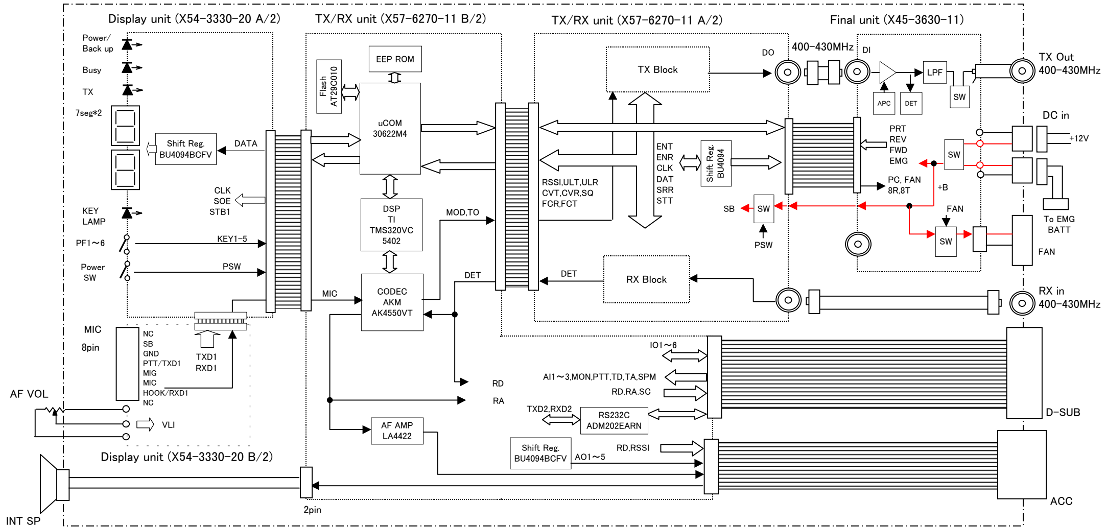
TKR-850K3 Block Diagram
