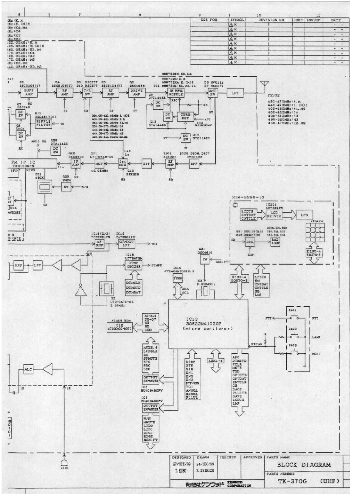
BLOCK DIAGRAM(RIGHT) Model Name:TK-370GK3/TK-360GK3 FCC ID:ALH29473130
