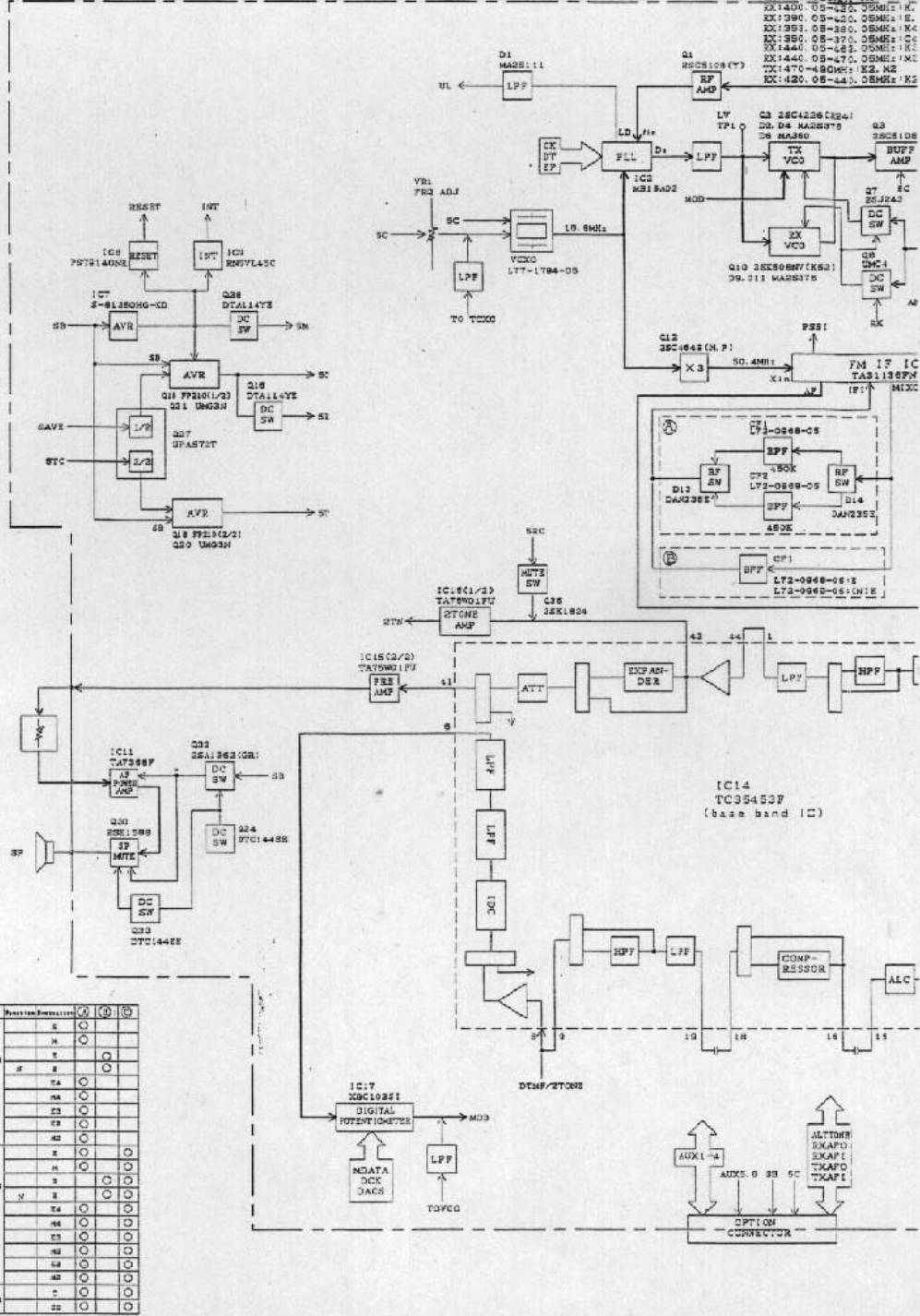
BLOCK DIAGRAM(Left) Model Name:TK-370GK3/TK-360GK3 FCC ID:ALH29473130
