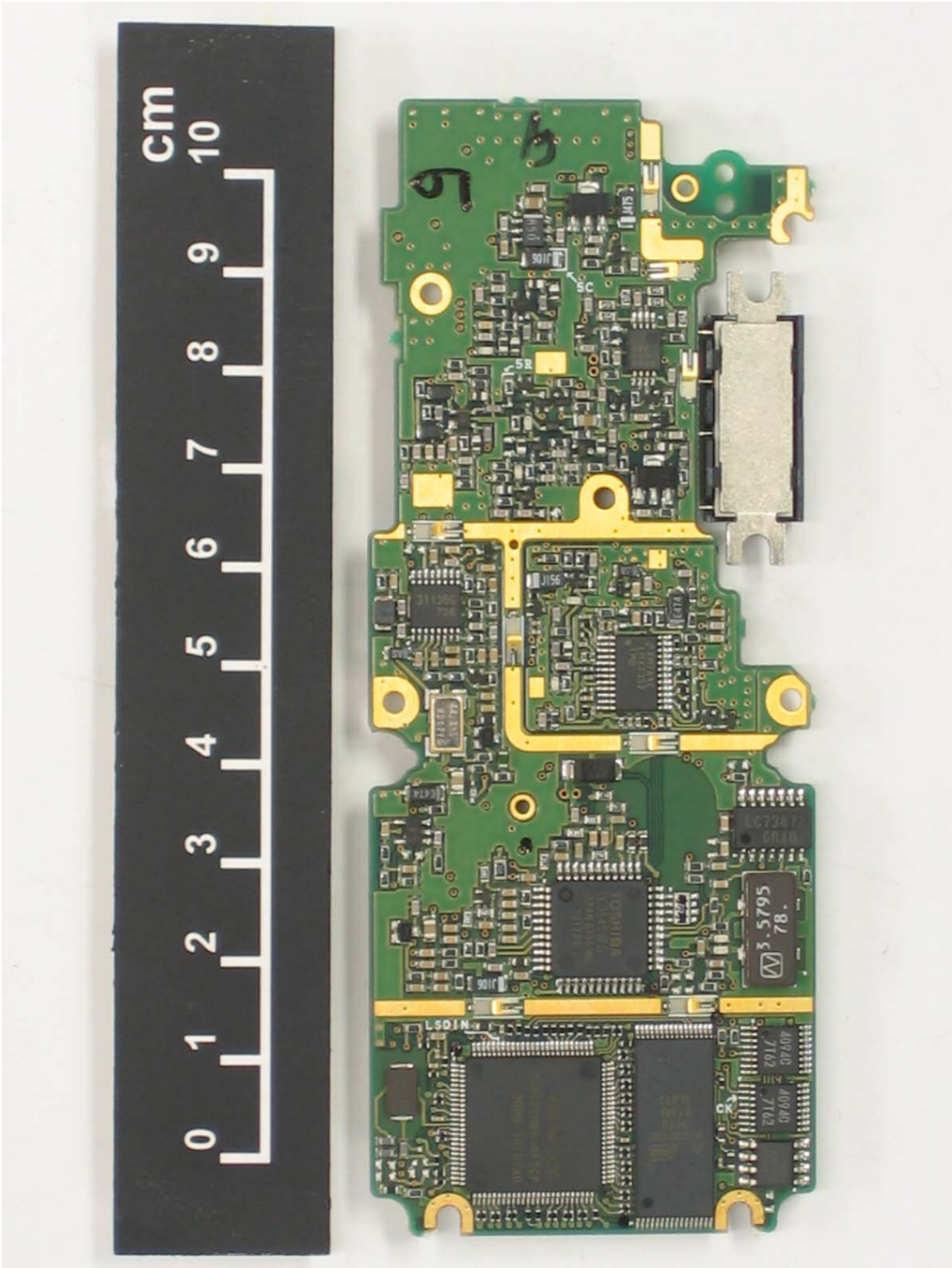
TXRX Foil Side View
