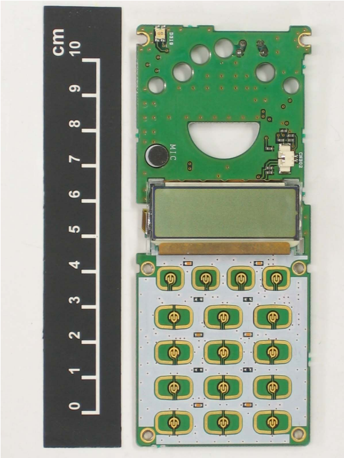
Display Component Side View
