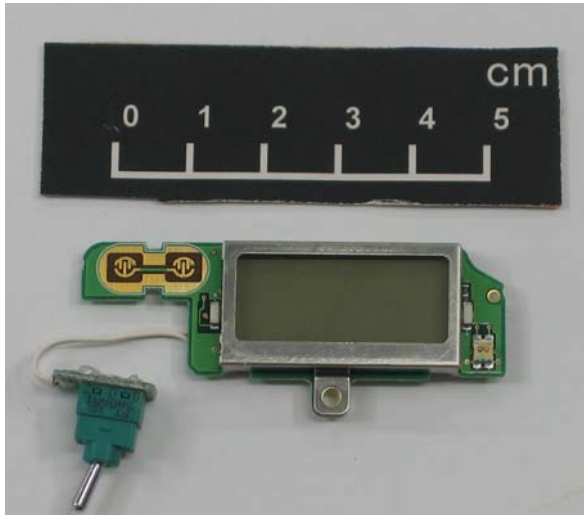
LCD Component Side View
