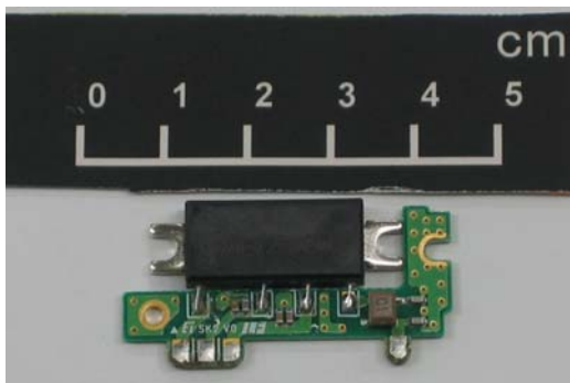
PA Component Side View
