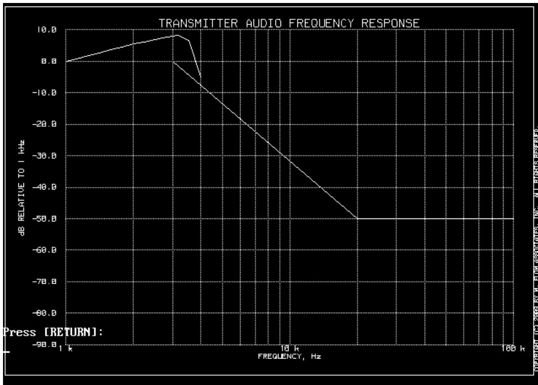
Low Pass Filter Response – 12.5 KHz BW
