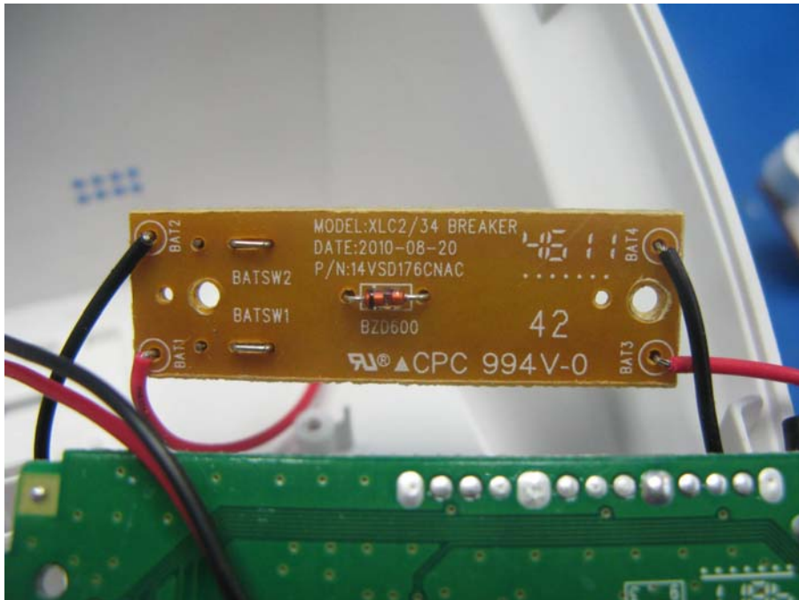
Base Unit Charging Board 2 PCB rear side
