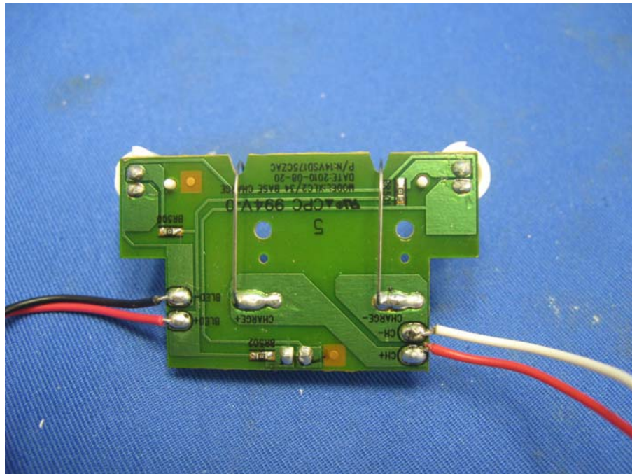
Base Unit Charging Board 1 PCB front side
