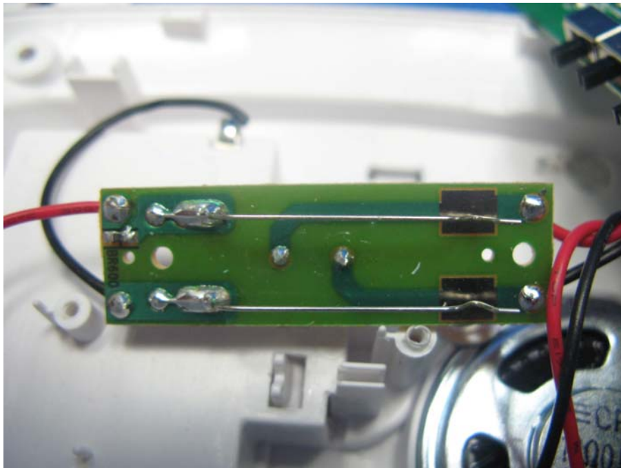
Base Unit Charging Board 2 PCB front side
