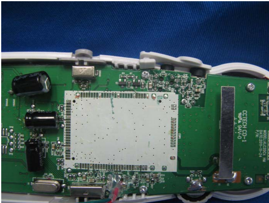
Handset Main PCB comp side (View 3)
