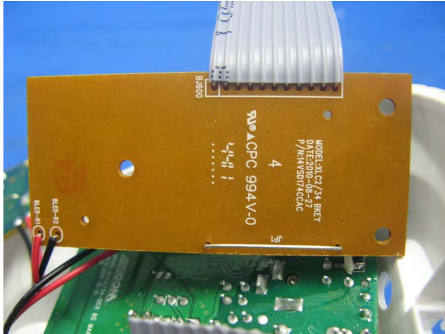
Base Unit Page Key rear side (View 2)
