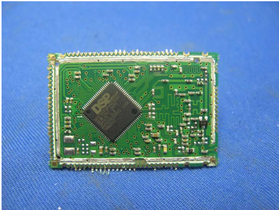
Base Unit RF Module comp side
