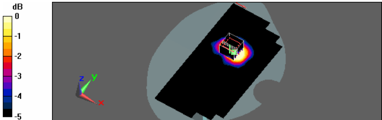
0 dB = 0.00803mW/g
